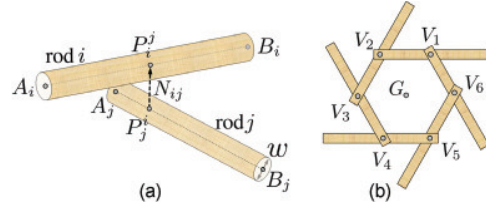
Figure 13: Notations used in the constraint definitions.
