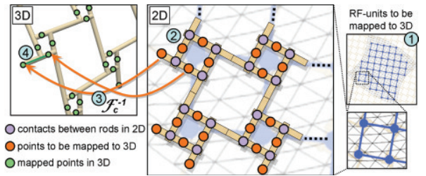
Figure 11: Initial placement of rods in 3D by \mathcal{F}_c^{-1} : 1) locate expected contact points (purple) between rods; 2) locate the related mid-points and endpoints (orange); 3) map these orange points from \mathcal{S} to 3D by \mathcal{F}_c^{-1} ; and 4) connect the mapped points (green) correspondingly to layout the rods in 3D.
