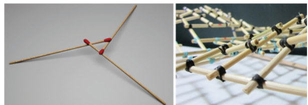
Figure 2: Left: A three rods reciprocal frame, as an RF-unit. Right: a large RF-structure made up of tied rods.
